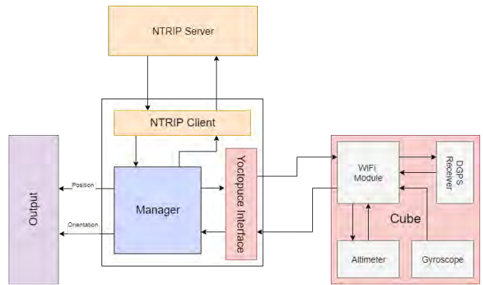
Figure 2: The general architecture of the system, showing its components and the communication of all parts.
