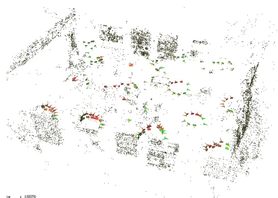
Figure 2: 3D segment . Figure (a) shows some of the input images used to create an initial sparse 3D reconstruction. Figure (b) shows two views of this reconstruction, triangulated natural feature points are shown as dark points, the camera positions and orientations of the input images are visualized by the coloured cones.
