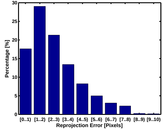
Figure 9: Reprojection error for inliers found during robust pose estimation. A reprojection error of \sim 10 pixels was allowed for an image size of 768x576 pixels.
