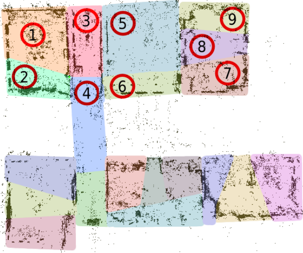
Figure 5: Representation of the reconstruction as separate PVS cells. The assignment of features to cells is color coded. The first 9 cells are indicated by the numbers inside red circles. Because we use cell based visibility, a PVS is created for each of these color coded cells and consists of an enumeration of all cells that are visible from one cell. For example, the PVS of cell 2 consists of cells (2, 1, 4).
