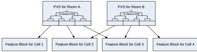
Figure 4: Two PVS with three cells each, sharing two of the cells.
