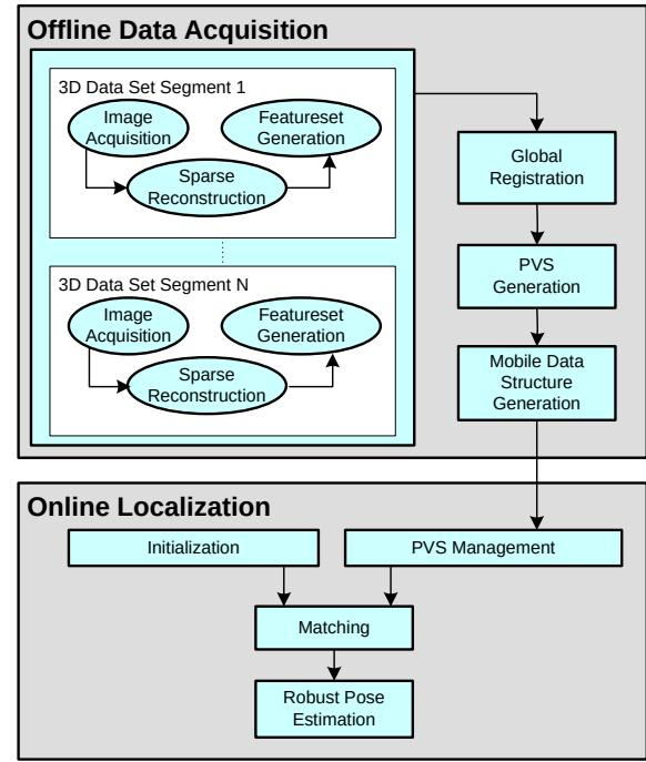
Figure 1: Work flow overview. The system can be divided into an of-line data acquisition and an online localization part. The offline data acquisition step creates globally registered 3D points with associated feature descriptors that are grouped into potentially visible sets. Optimized representations of this data are used on the mobile phone to localize the user efficiently.
