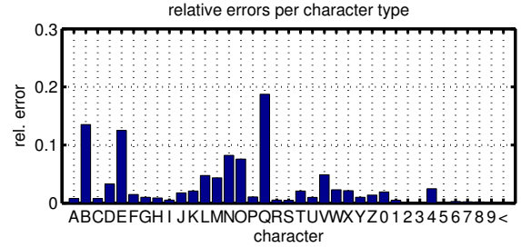
Figure 12: Errors for individual characters: In most cases, the characters B, E and Q are confused with others. Note: Individual errors are given relative to the sum of all errors across all characters.
