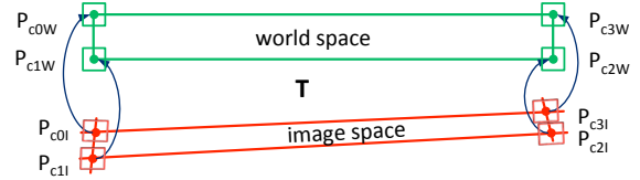
Figure 6: Rectification of Characters: First, a global transformation T is estimated using intersections points of fitted lines in image space and the corresponding world coordinates. Then, a local transformation can be estimated per character, which is then used for patch warping.
